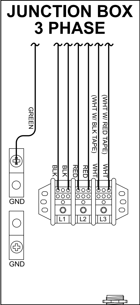
UNIT WIRED 3 PHASE FROM FACTORY
