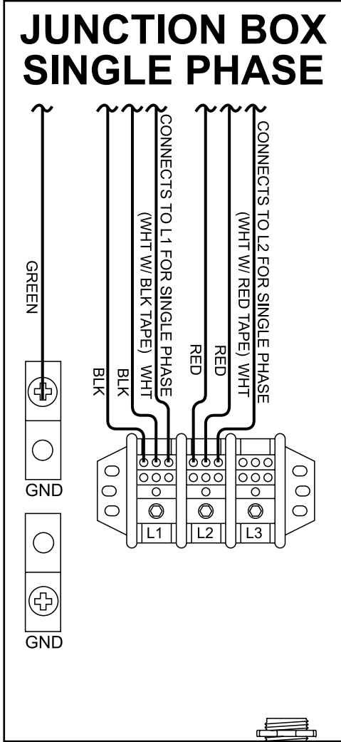
IF REWIRED FOR SINGLE PHASE - CURRENT @220VAC IS 69A
